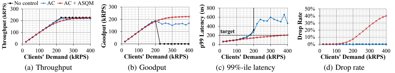
Figure 11: Performance of Protego by incrementally applying performance-driven admission control (AC) and ASQM with the synthetic application with 10 \mu\text{s} average service time
